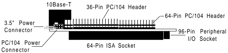
Side View of QTB/104 Viewed from Bus Side
